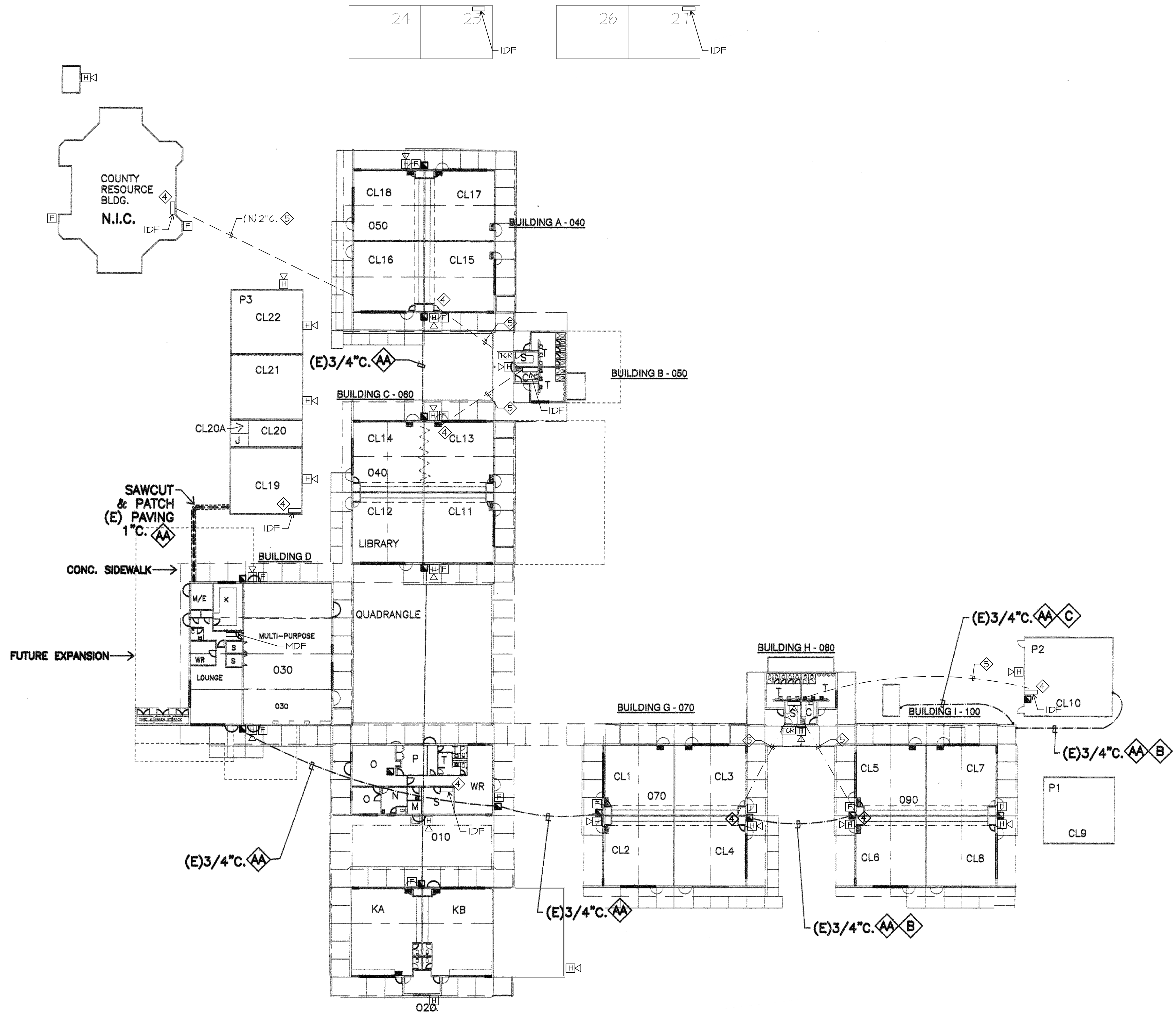
EXISTING FIRE ALARM SITE PLAN
