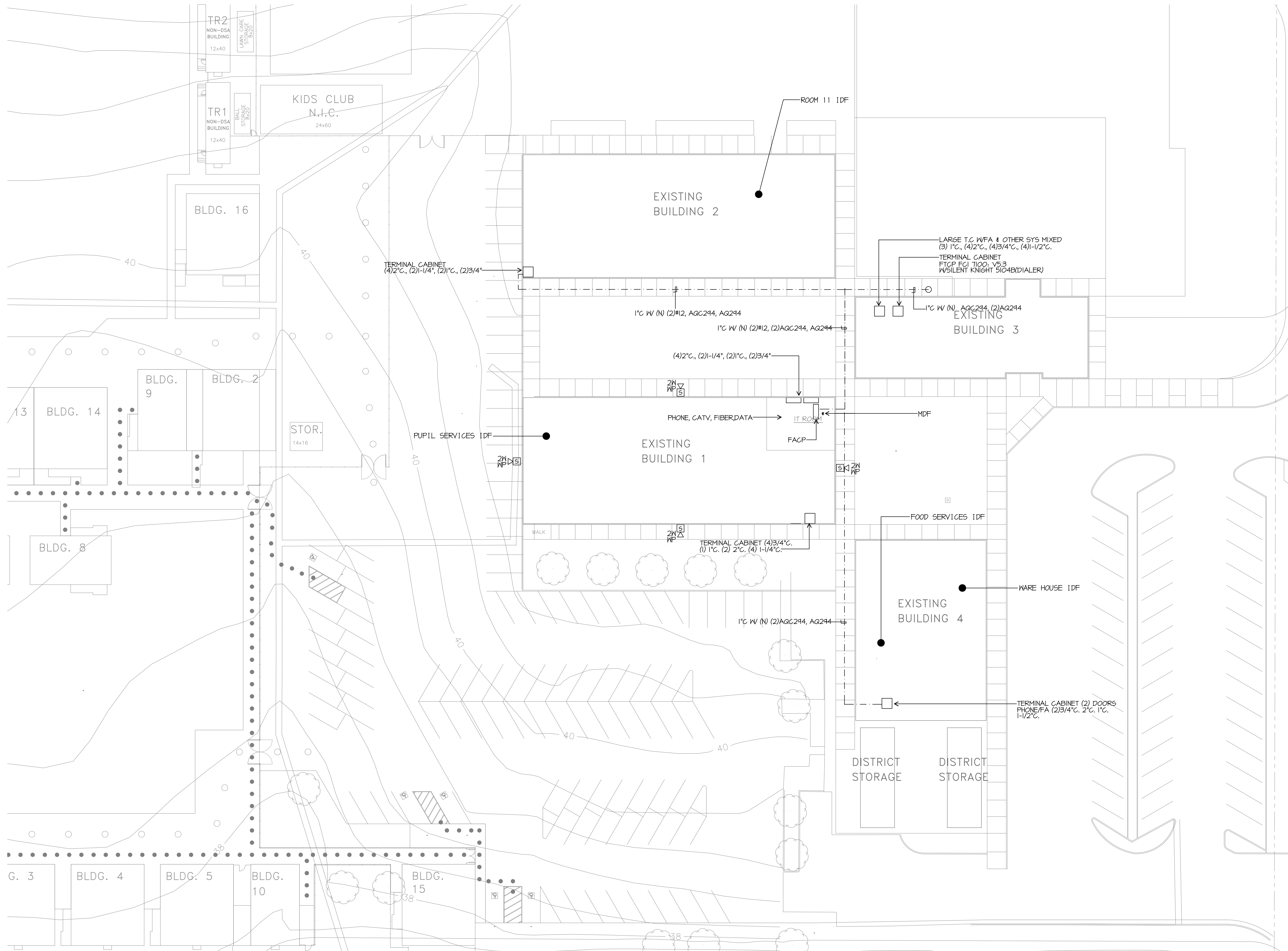
EXISTING FIRE ALARM SITE PLAN
